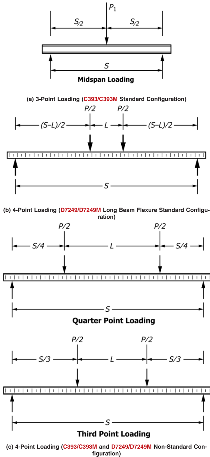
FIG. 1 Loading Configurations
